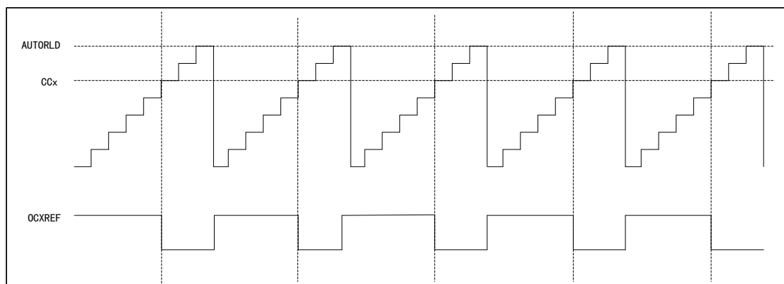
Figure 45 PWM1 Count-up Mode Timing Diagram
