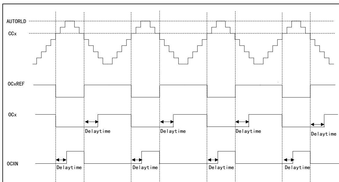
Figure 82 Complementary Output of Insertion with Dead-time
